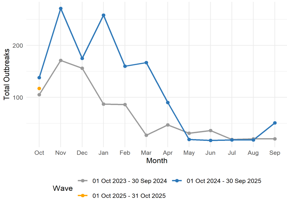
Figure 1a - Northern hemisphere
