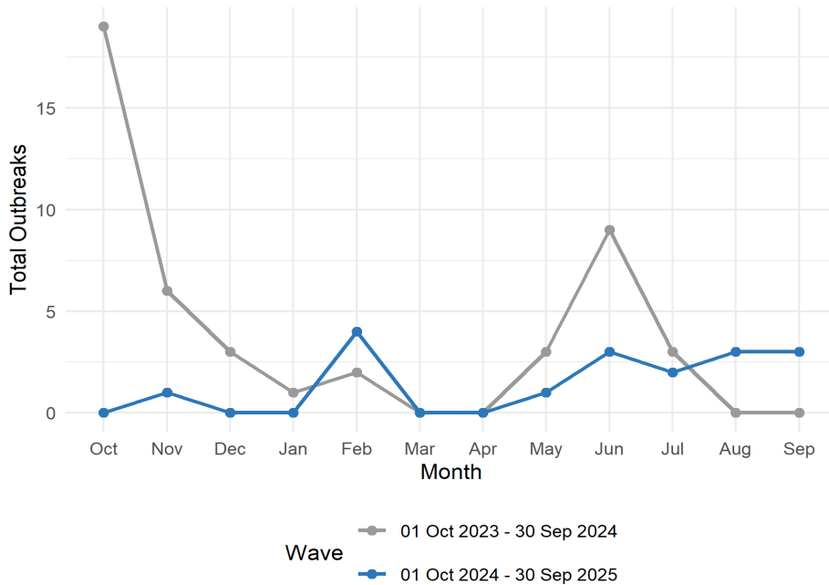
Figure 1b - Southern hemisphere
