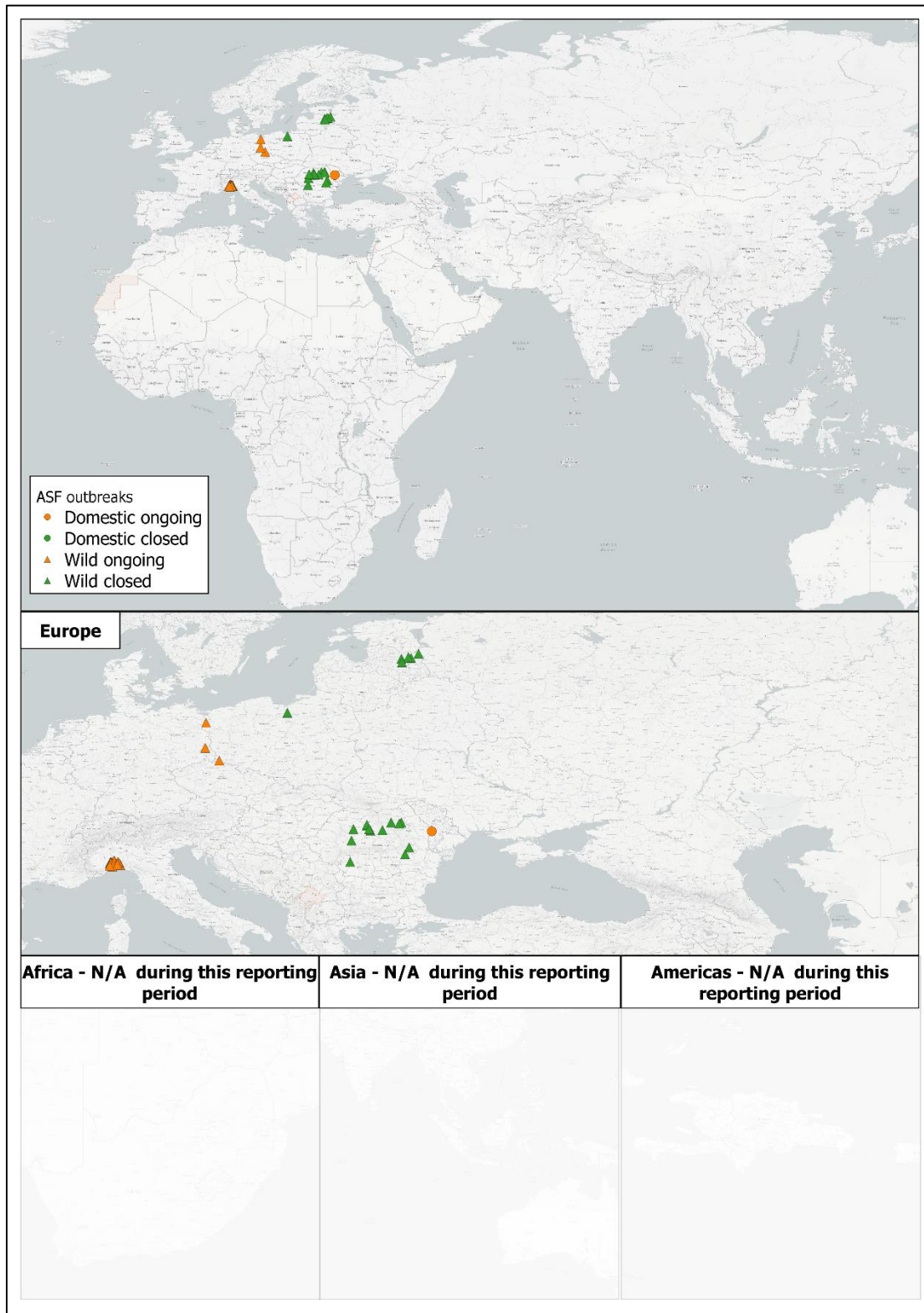
Figure 1: Map of ASF outbreaks which started during 17 Feb 2023 – 02 Mar 2023 in domestic animals and wildlife. Zoomed views of areas where updates occurred in the last period are provided as well.
