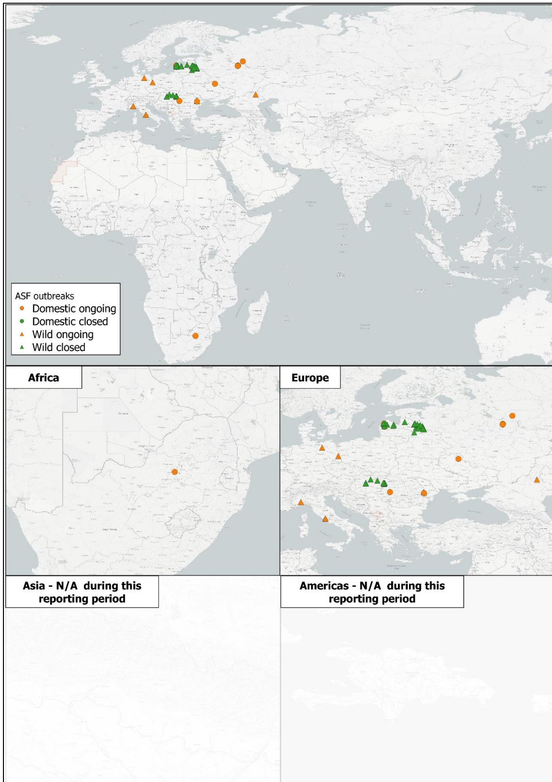
Figure 1: Map of ASF outbreaks which started during 08 July – 21 July 2022 in domestic animals and wildlife. Zoomed views of areas where updates occurred in the last period are provided as well.
