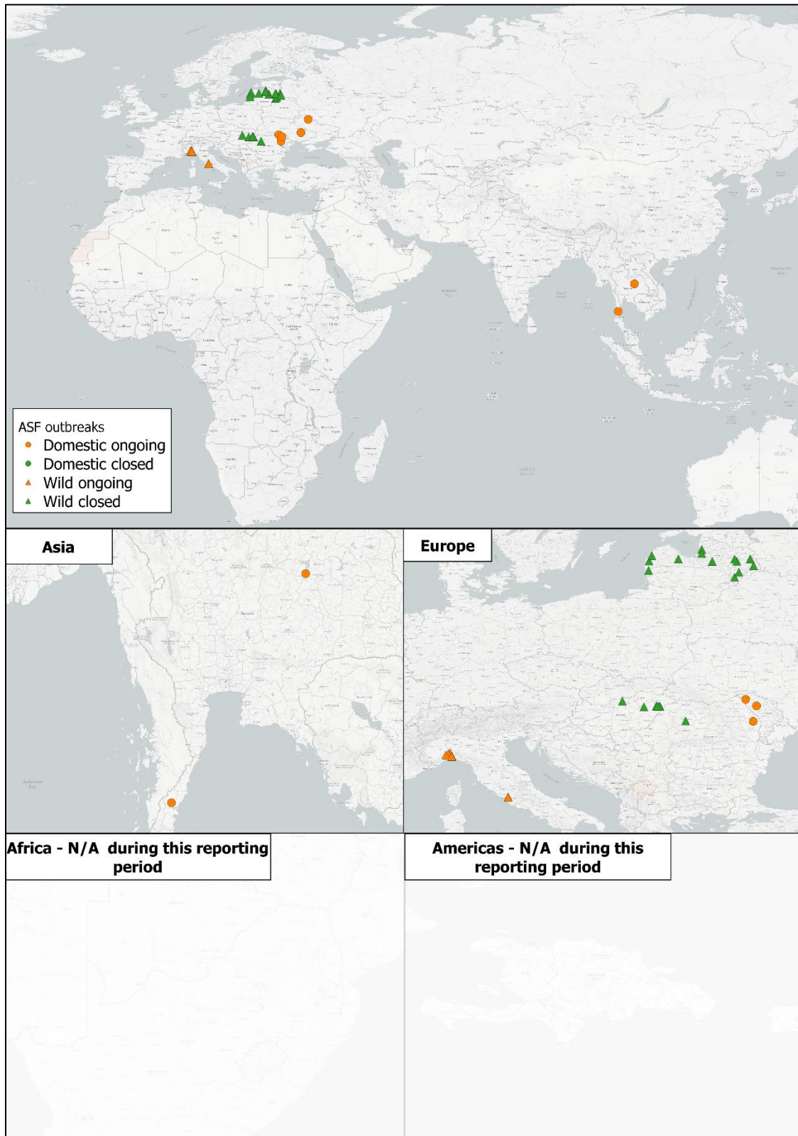
Figure 1: Map of ASF outbreaks which started during 10 June – 23 June 2022 in domestic animals and wildlife. Zoomed views of areas where updates occurred in the last period are provided as well.
