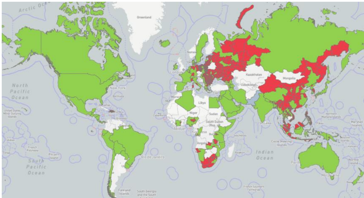
Figure 2. Map of the world displaying the presence of ASF by Administrative divisions (2020 – 23/06/2022)
